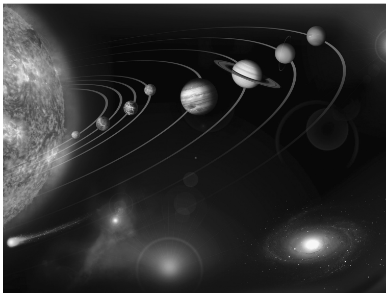
FIGURE I.4 A schematic view of the Solar System (not to scale), with the terrestrial planets close to the Sun and the giant planets at further distances, beyond the main asteroid belt. A comet is shown near the orbits of Jupiter and Saturn. For colour version, see plates section. (Image courtesy of NASA/JPL.)
